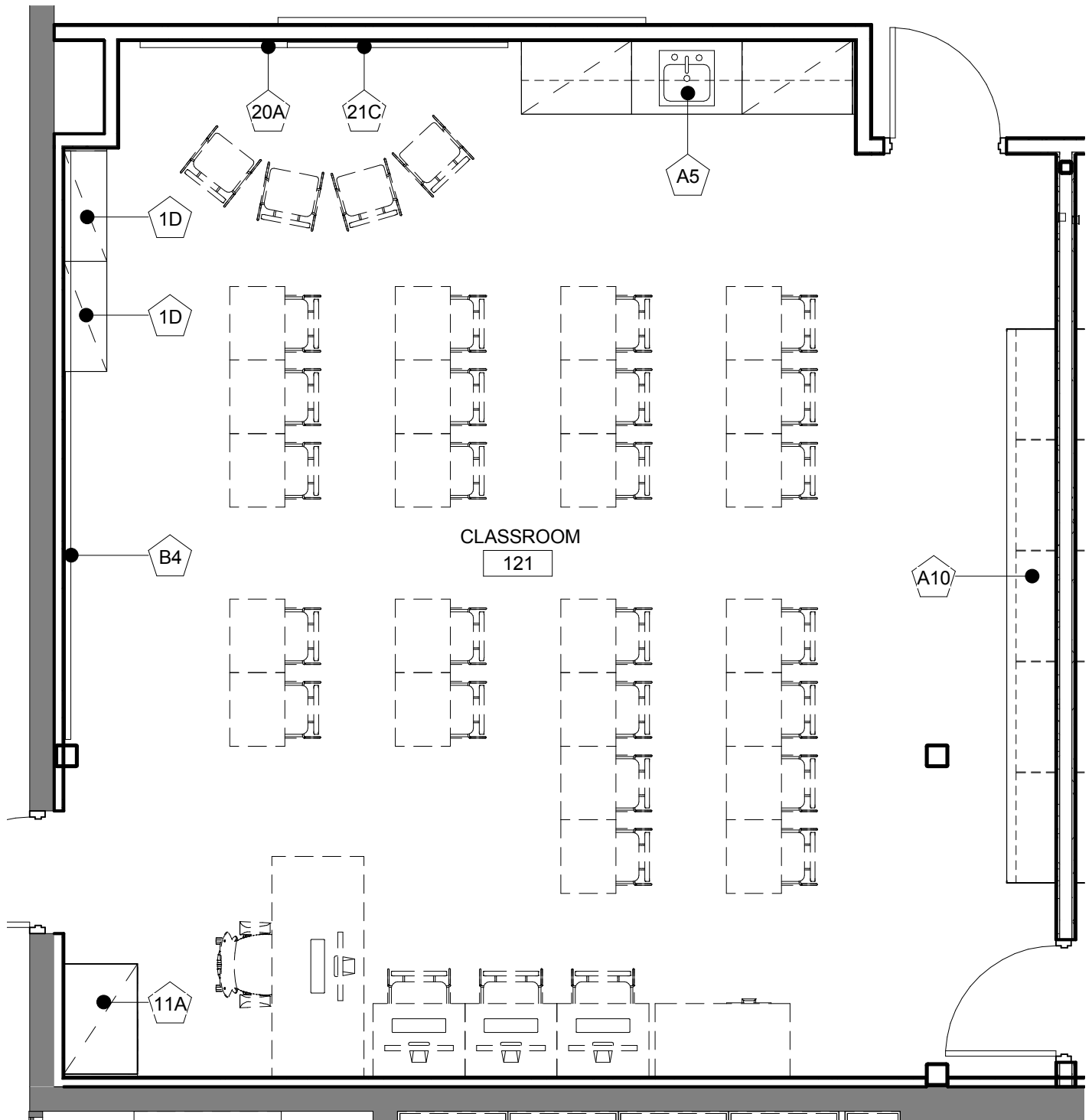
1 PRIMARY CLASSROOM 1/4" = 1'-0"
