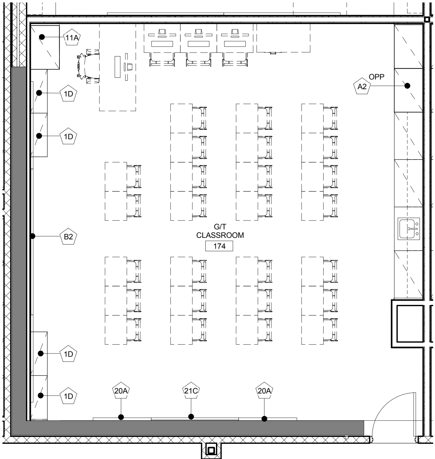
1 GT CLASSROOM 1/4" = 1'-0"
