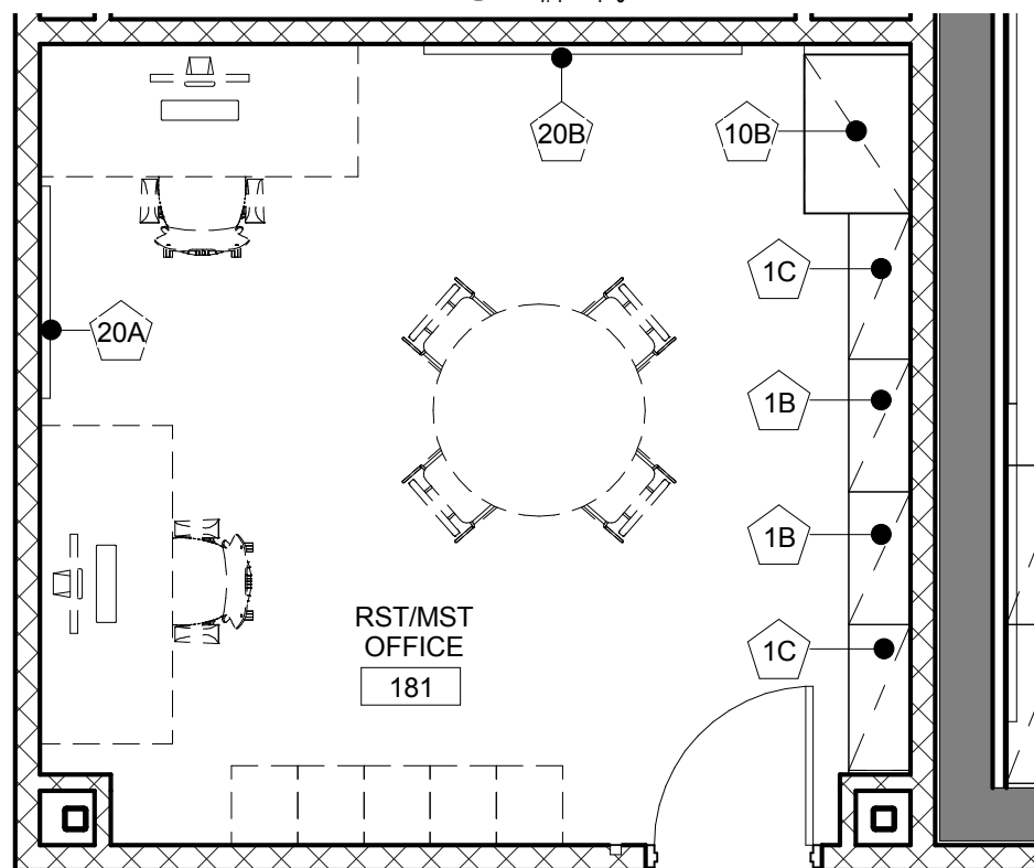
3 RST/MST OFFICE 1/4" = 1'-0"
