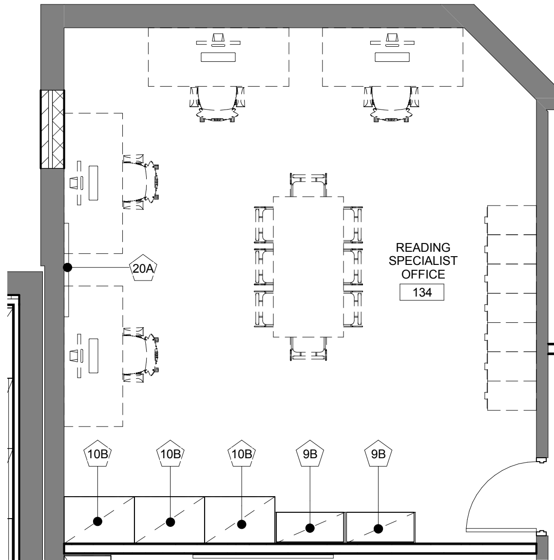
1 READING SPECIALIST 1/4" = 1'-0"
