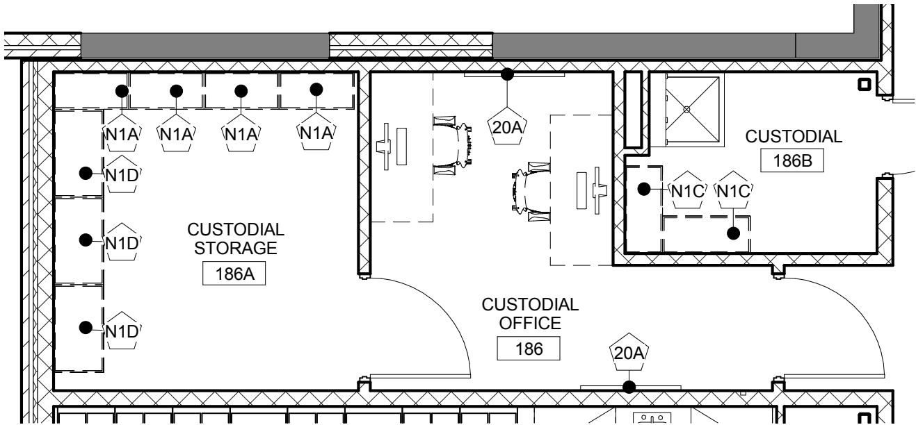
2 CUSTODIAL OFFICE AND STORAGE 3/16" = 1'-0"
