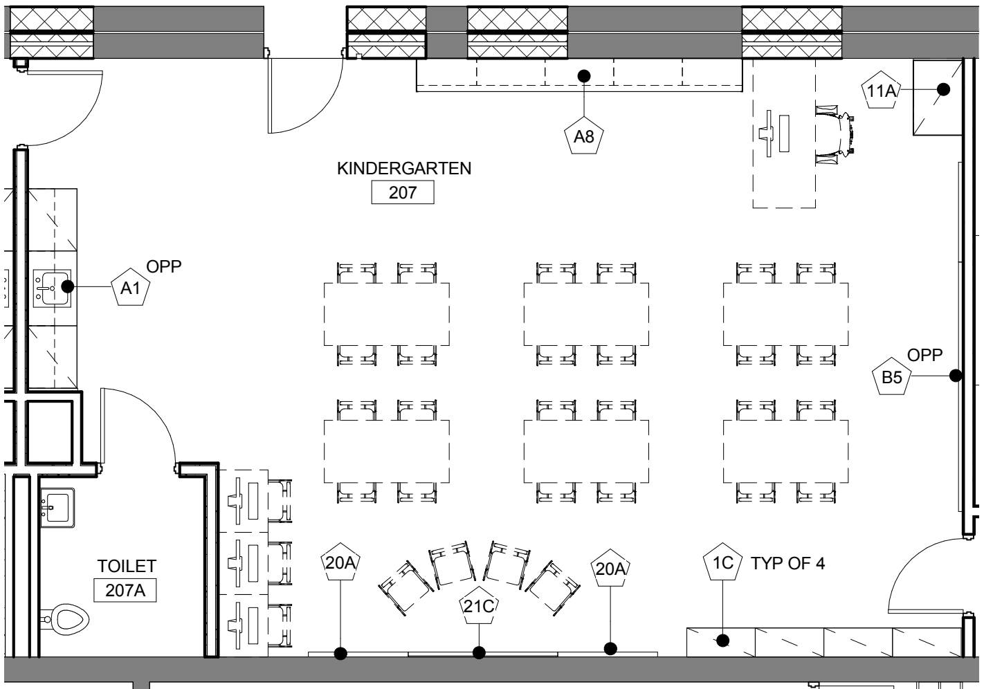
1 KINDERGARTEN 3/16" = 1'-0"
