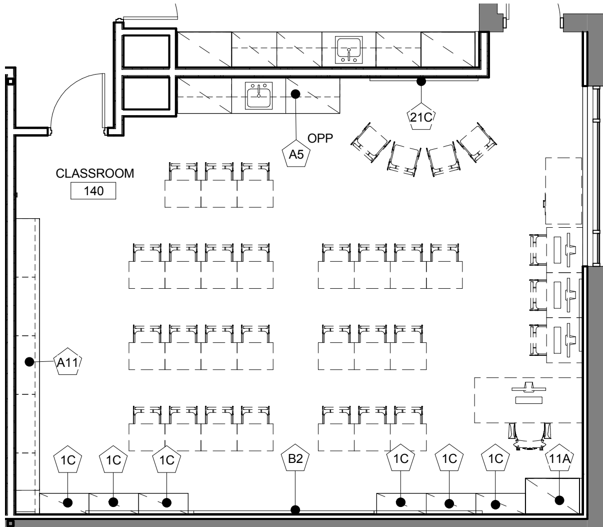
1 INTERMEDIATE CLASSROOM 3/16" = 1'-0"
