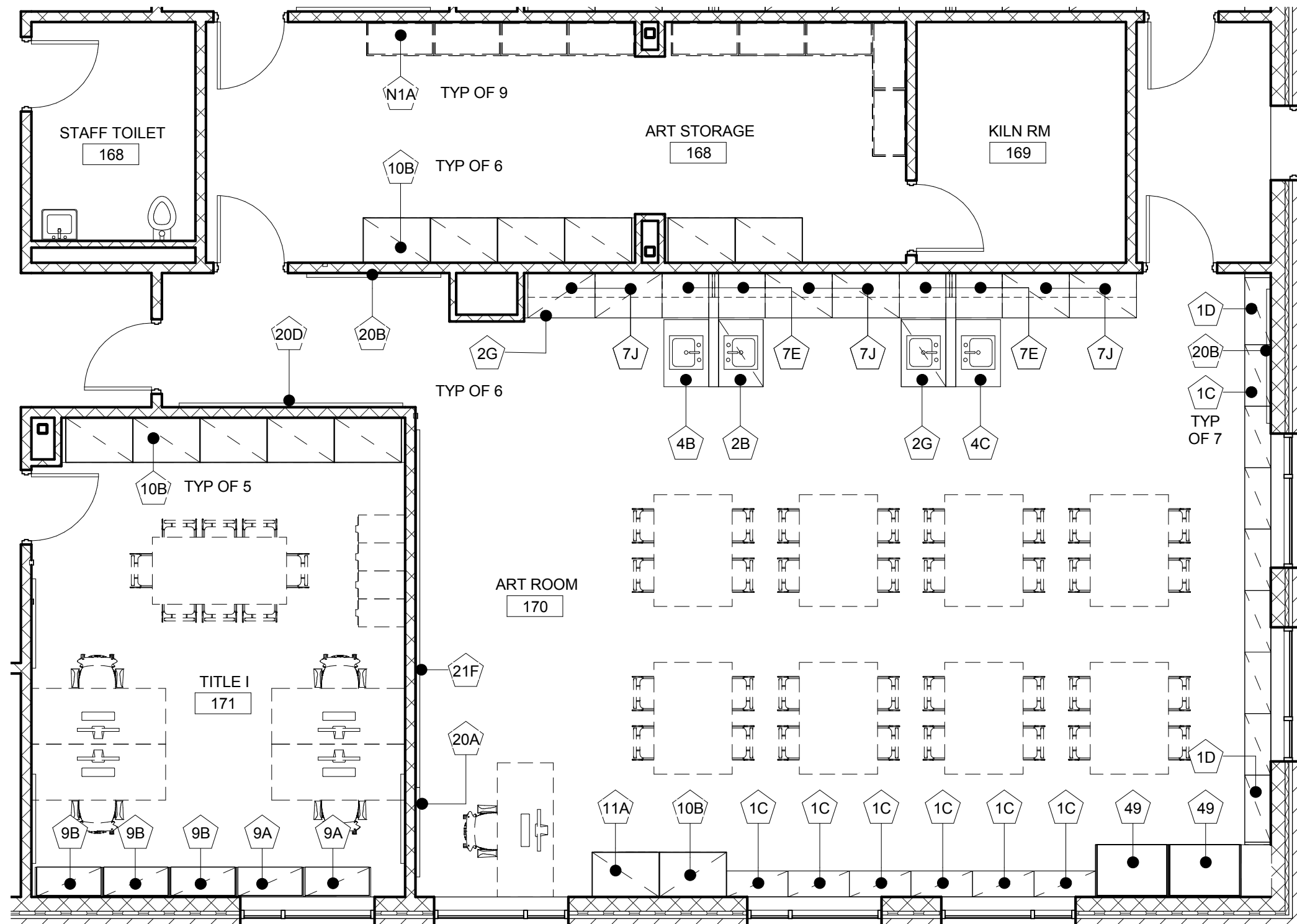
② ART ROOM/ TITLE 1 3/16" = 1'-0"
