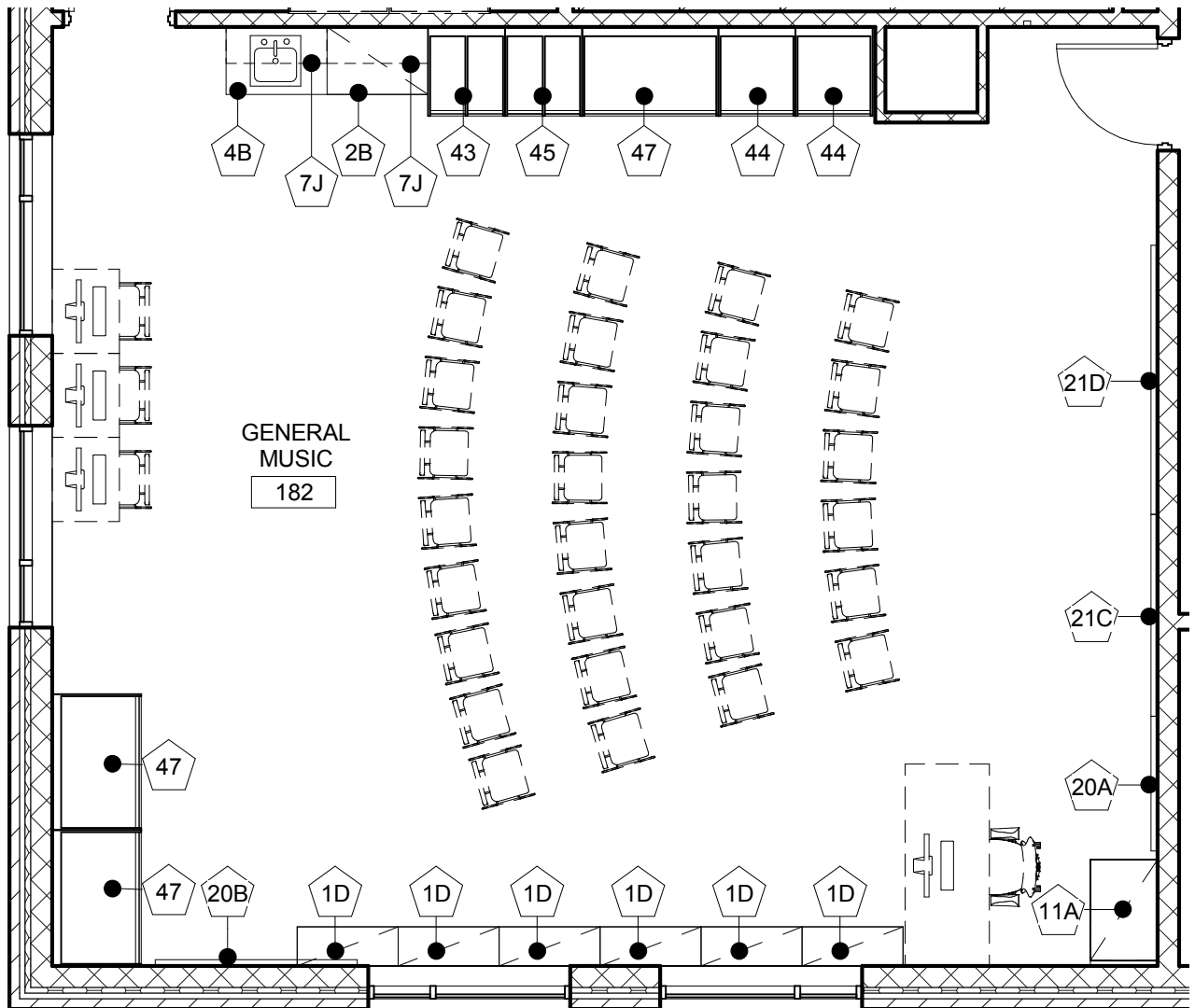
1 GENERAL MUSIC 3/16" = 1'-0"
